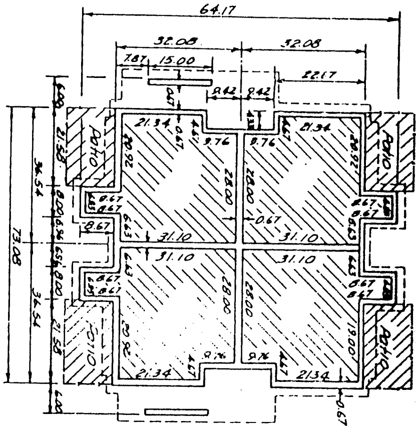
PLAN VIEW
